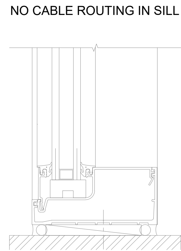
DETAIL 3 SILL
