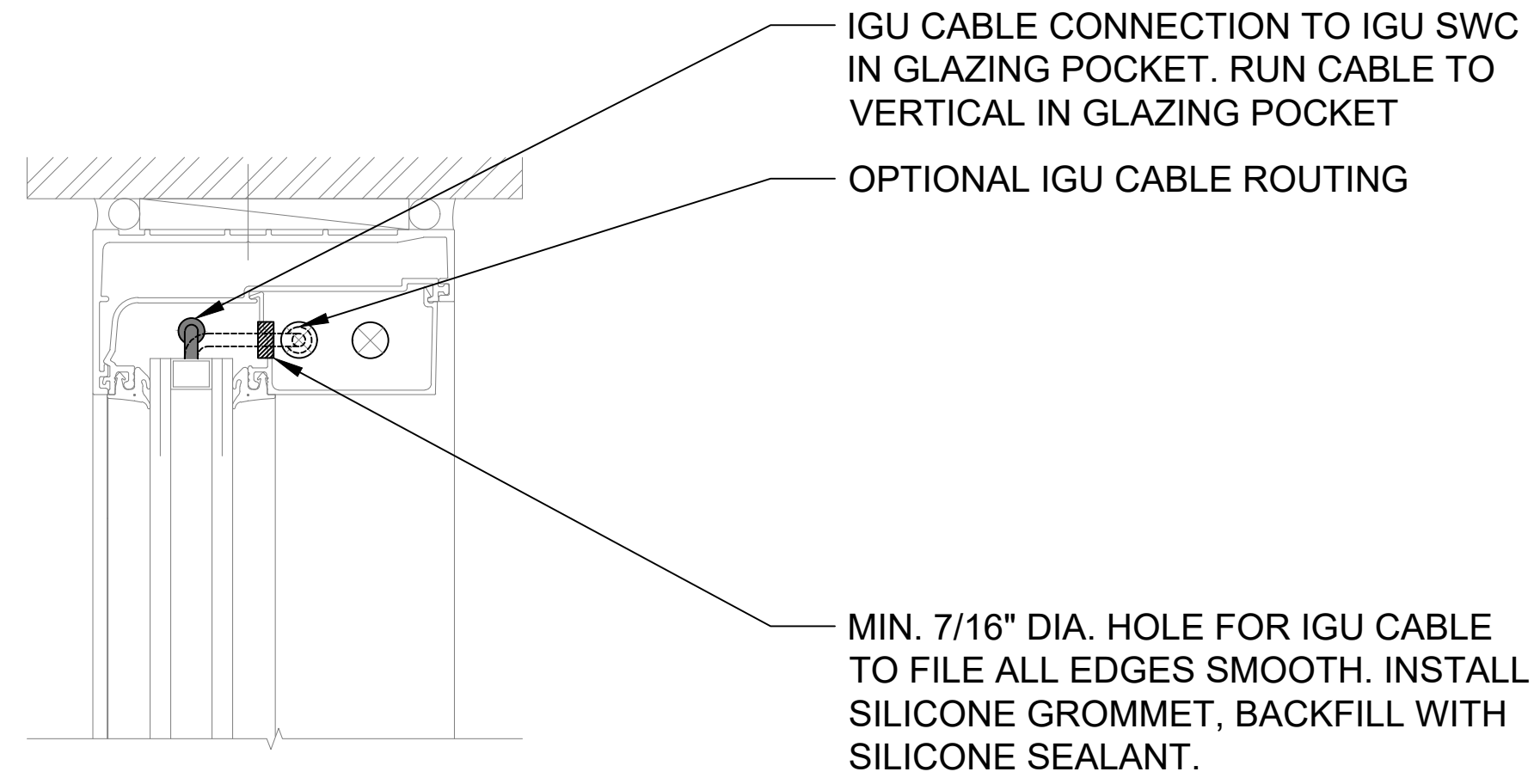
DETAIL 1 HEAD
