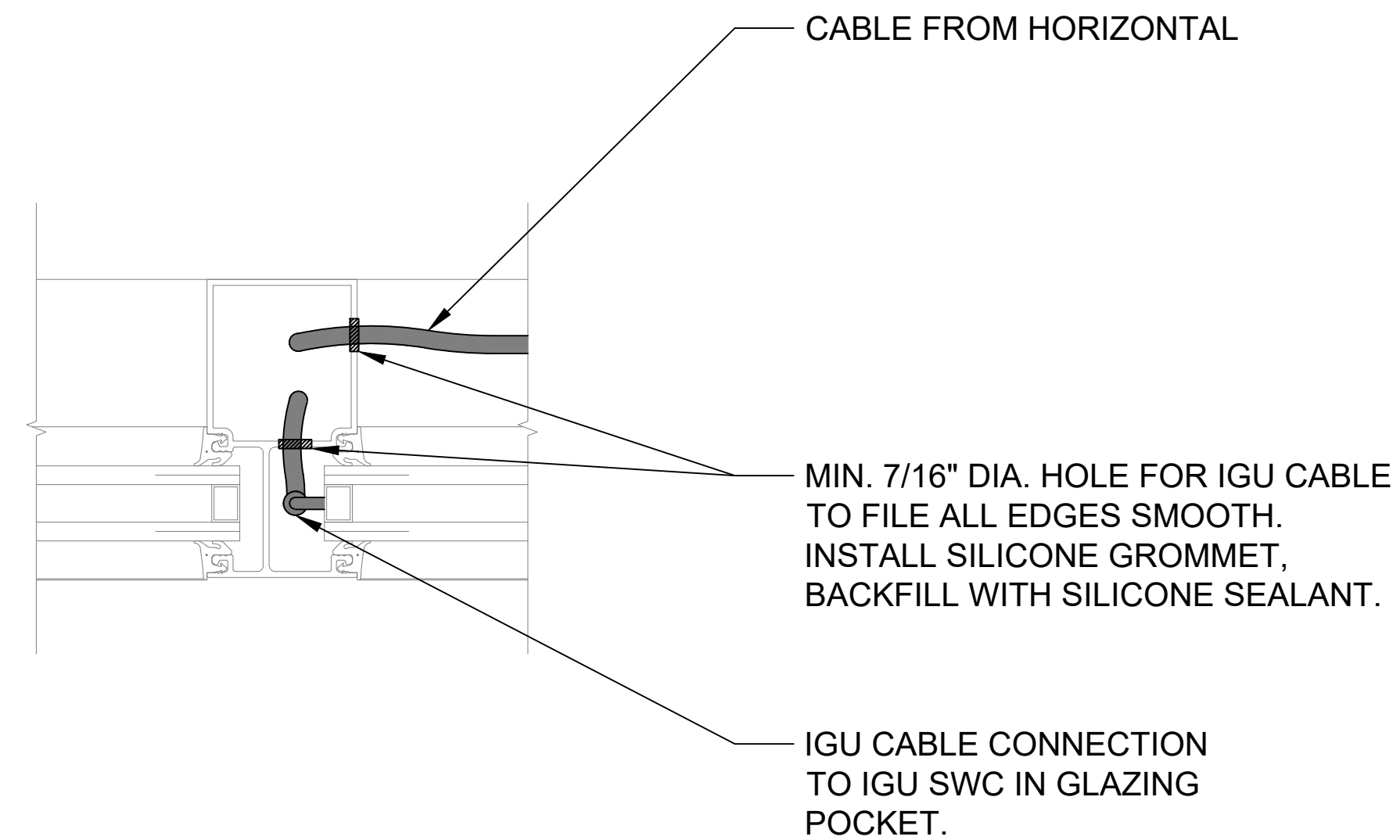
DETAIL 5 VERTICAL MULLION
