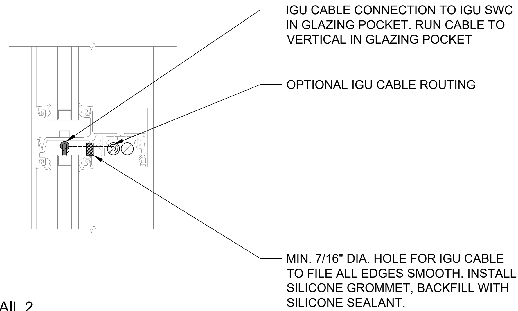
DETAIL 2 HORIZONTAL MULLION
